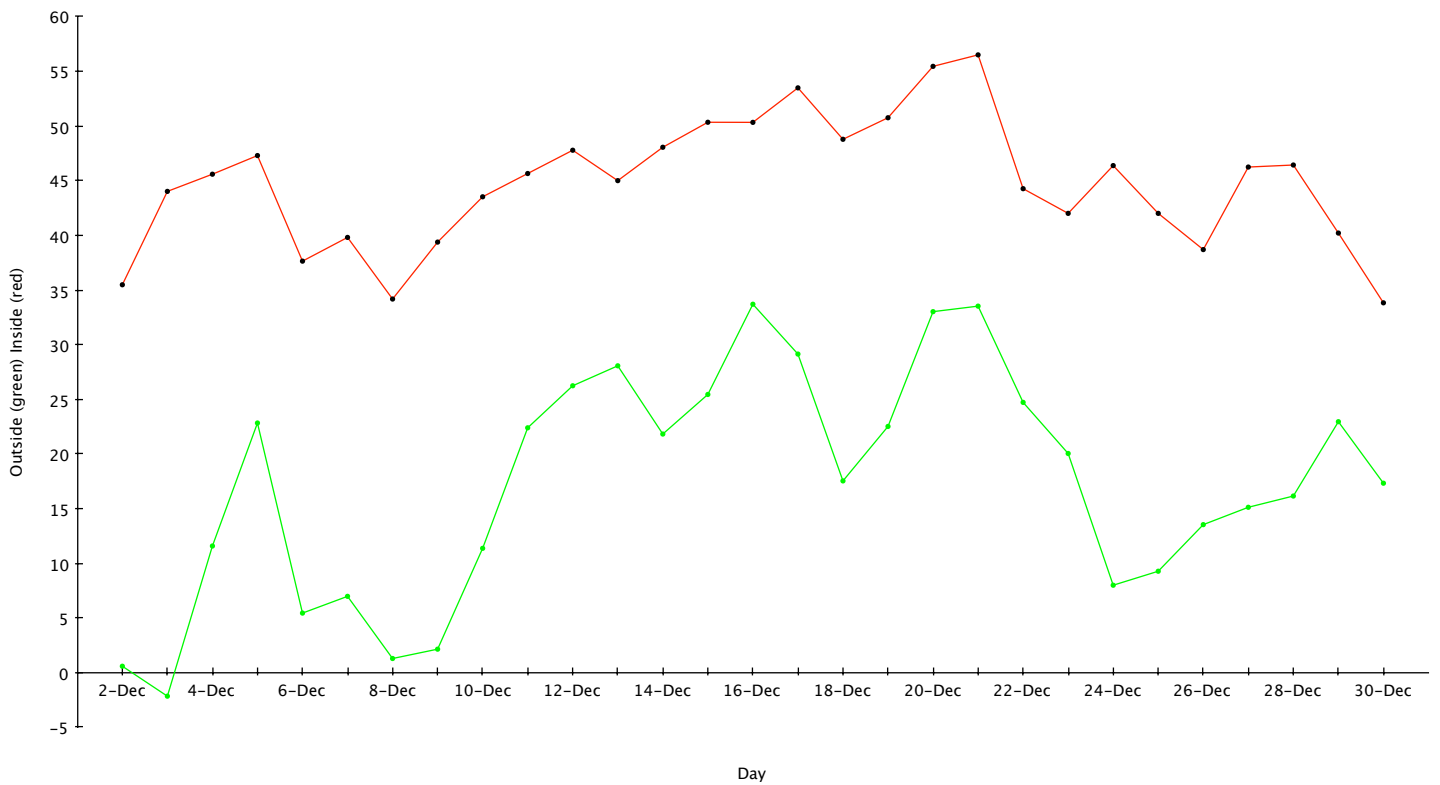
Average daily temperature Outside (green) and Inside (red) the dome greenhouse Dec '09
